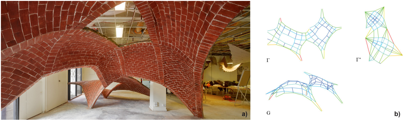
Figure 4. Workshop at MADA, Melbourne, 2013, instructed by P. Block (ETH Zurich), J. Bellamy (Re-vault), T. Schork (MADA) and D. Van Horne (Grimshaw Architects), a ) result (Photo: Peter Bennetts), b ) form diagram ( \Gamma ), force diagram ( \Gamma^* ) and 3D thrust network (G) (RhinoVault).
