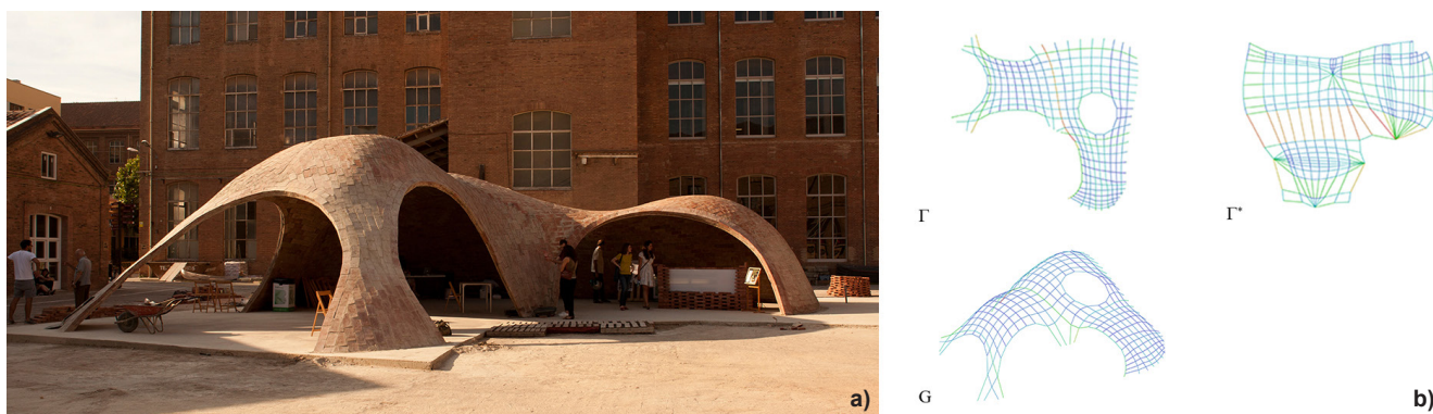
Figure 3. “Brick-topia”, Map13 Barcelona, 2013, a) finished vault (Photo: Manuel de Lózar & Paula López), b) form diagram ( \Gamma ), force diagram ( \Gamma^* ) and 3D thrust network (G) (RhinoVault).
